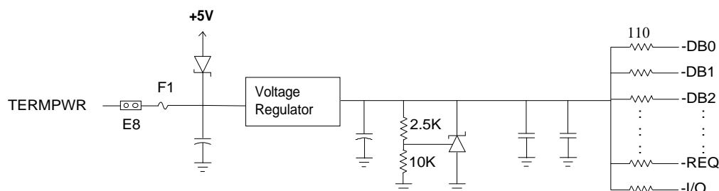
Figure 5-2 Terminator Equivalent Circuit
