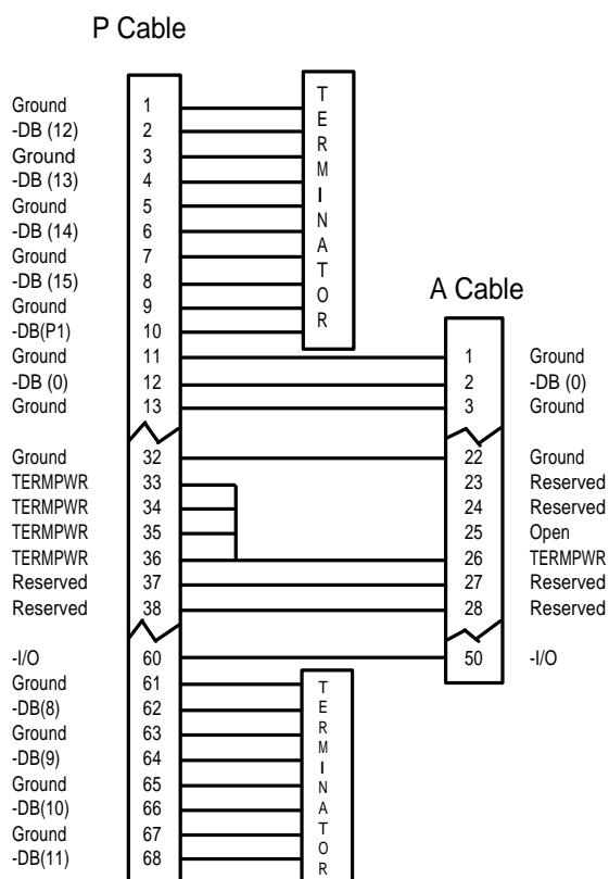
Figure 4-9 Wide-to-Narrow Adapter
