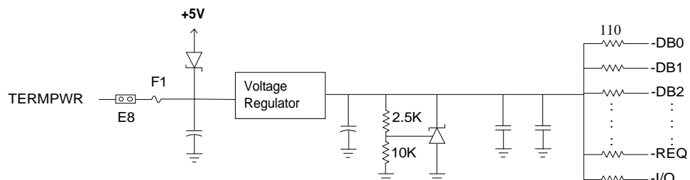
Terminator Equivalent Circuit
