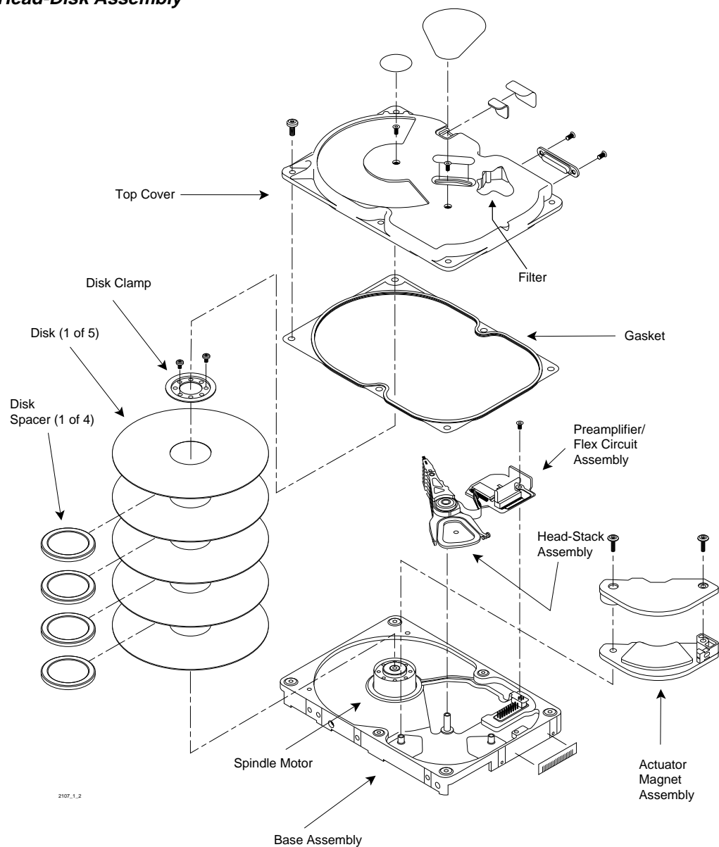
Figure 1-2 Head-Disk Assembly
