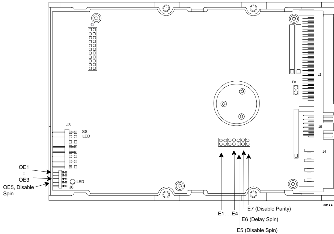
Figure 4-6 Jumper Locations
