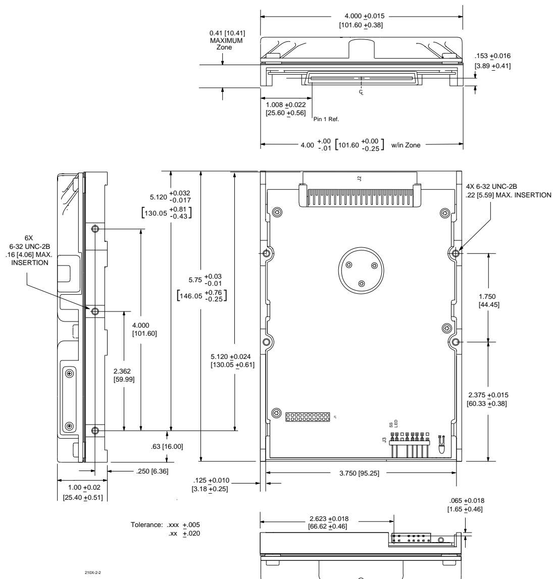
Figure 2-2 The Drive's Physical Dimensions
