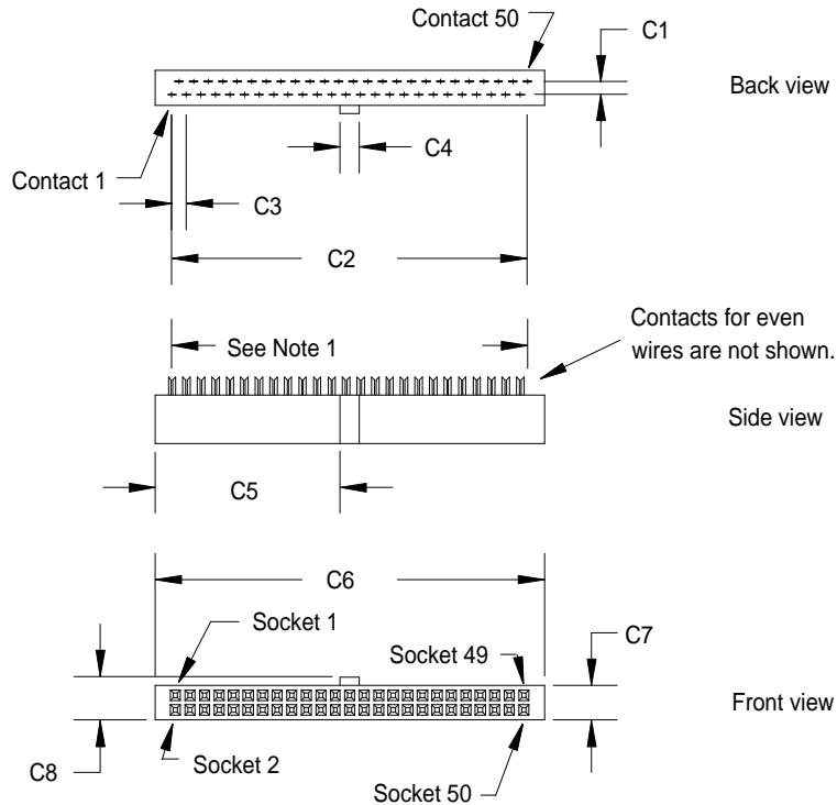
Figure 5-2 A-Cable Connector
