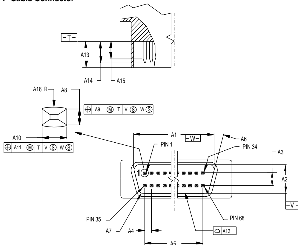
Figure 5-4 P-Cable Connector
