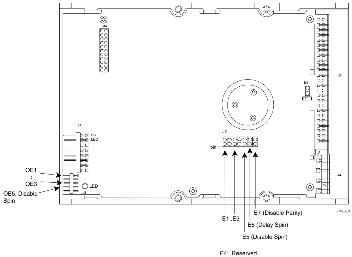
Figure 4-3 Jumper Locations
